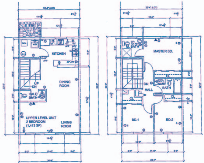
SECOND FLOOR 660 SF
