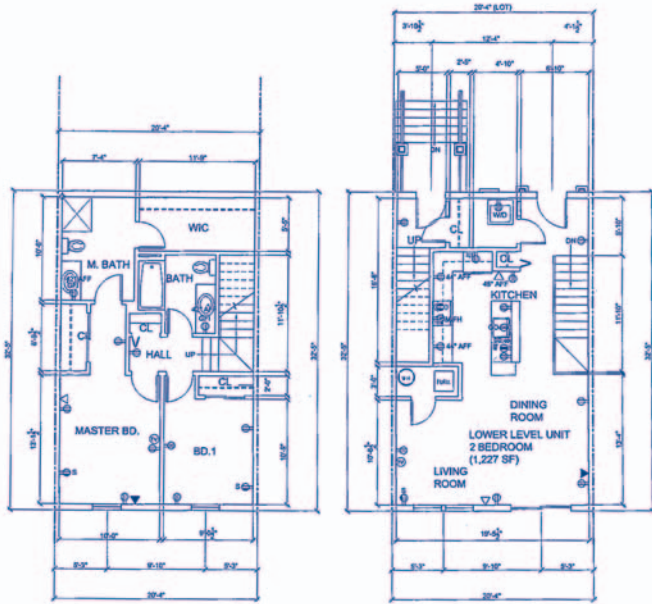
GROUND FLOOR 660 SF
